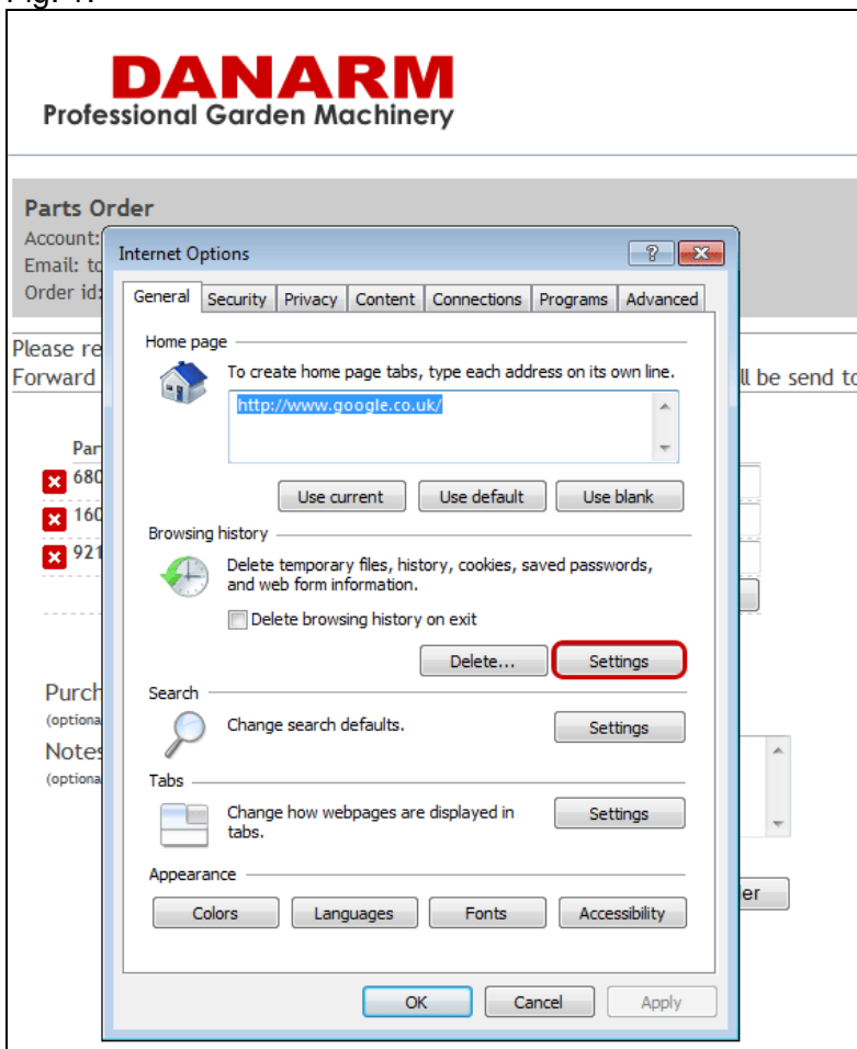
Fig 1: Internet Options
